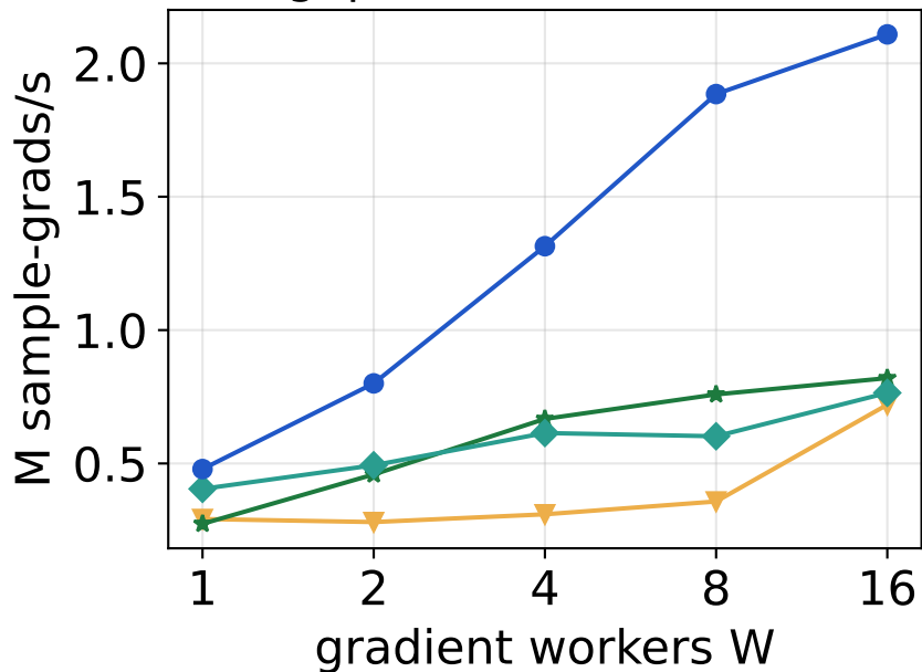
Throughput vs workers W (600k)
